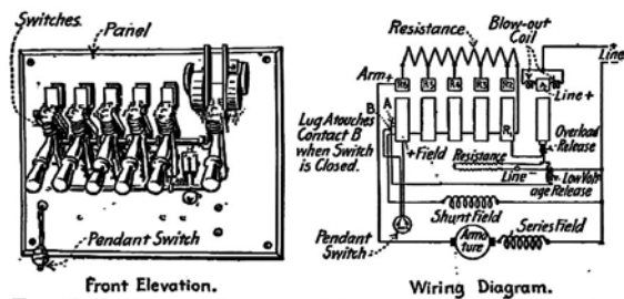
Fig. 97.—Multi-switch starter (single-pole starter is shown).
