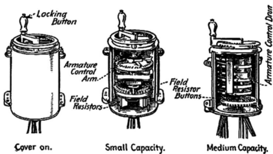
FIG. 91.—Machine-tool controller.
