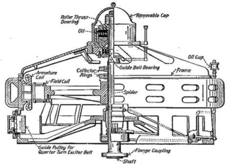
FIG. 172.—Sectional elevation of an Electrical Machinery Company vertical waterwheel generator. (See Fig. 173 for a photographic reproduction.)
