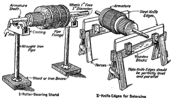
Fig. 153.—Roller-bearing armature stand and knife-edge leveling rig.
